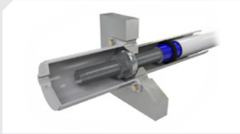
Head for permanent ground anchor
