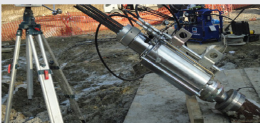
Tensioning jack
