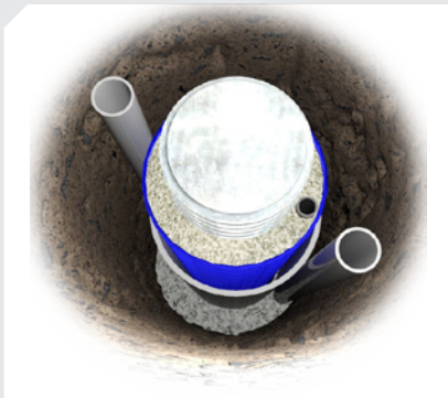
Cross-section of the free length of the anchor with an injection pipe
