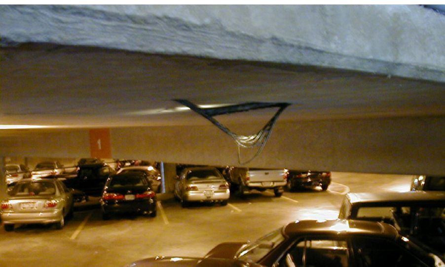
Peeling following a broken greased sheathed strand
